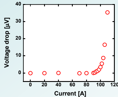
A practical high-temperature superconducting wire, Bi-2223 tape
